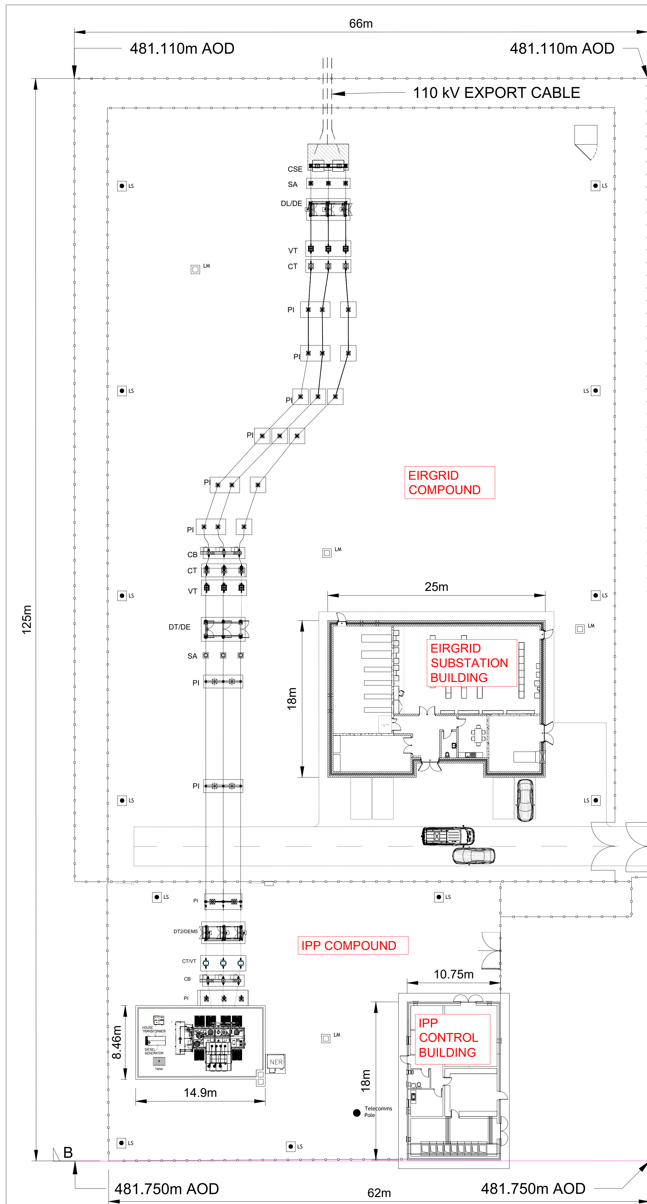
SUBSTATION PLAN SCALE 1:500
